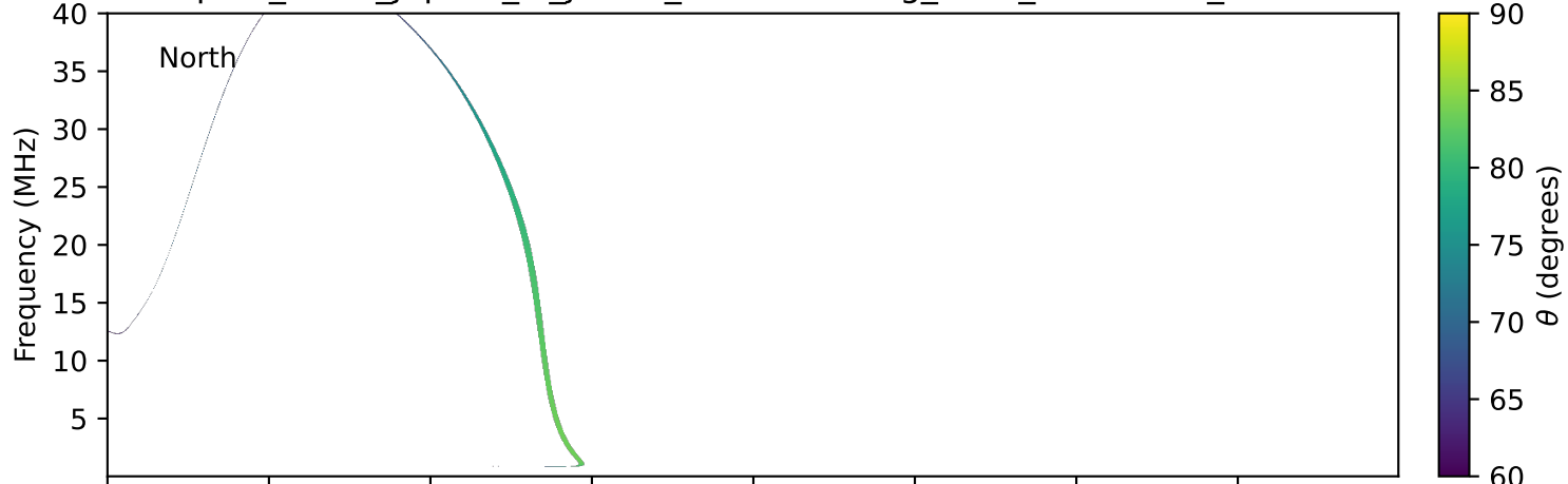
expres_earth_jupiter_io_jrm09_lossc-wid1deg_3kev_19950705_v11.cdf
