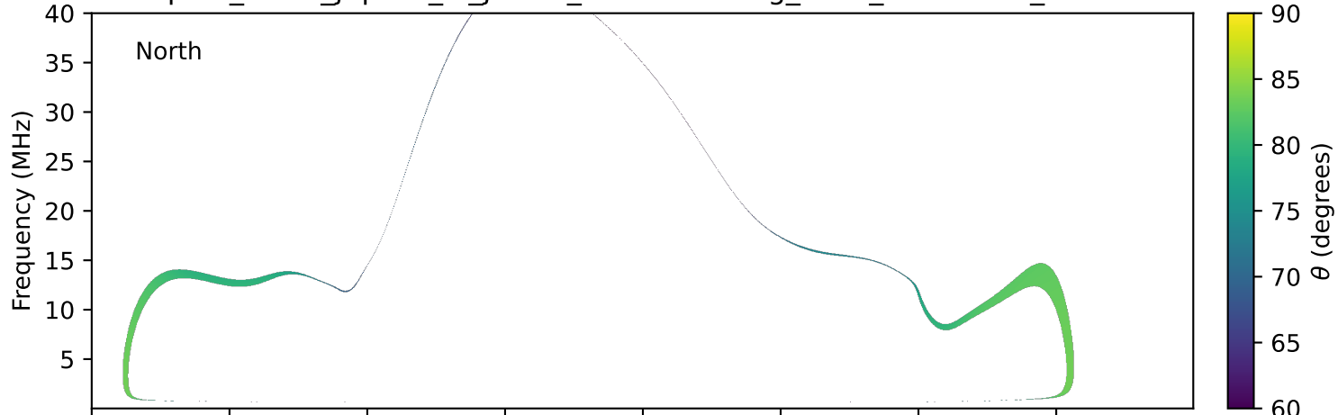
expres_earth_jupiter_io_jrm09_lossc-wid1deg_3kev_19950701_v11.cdf
