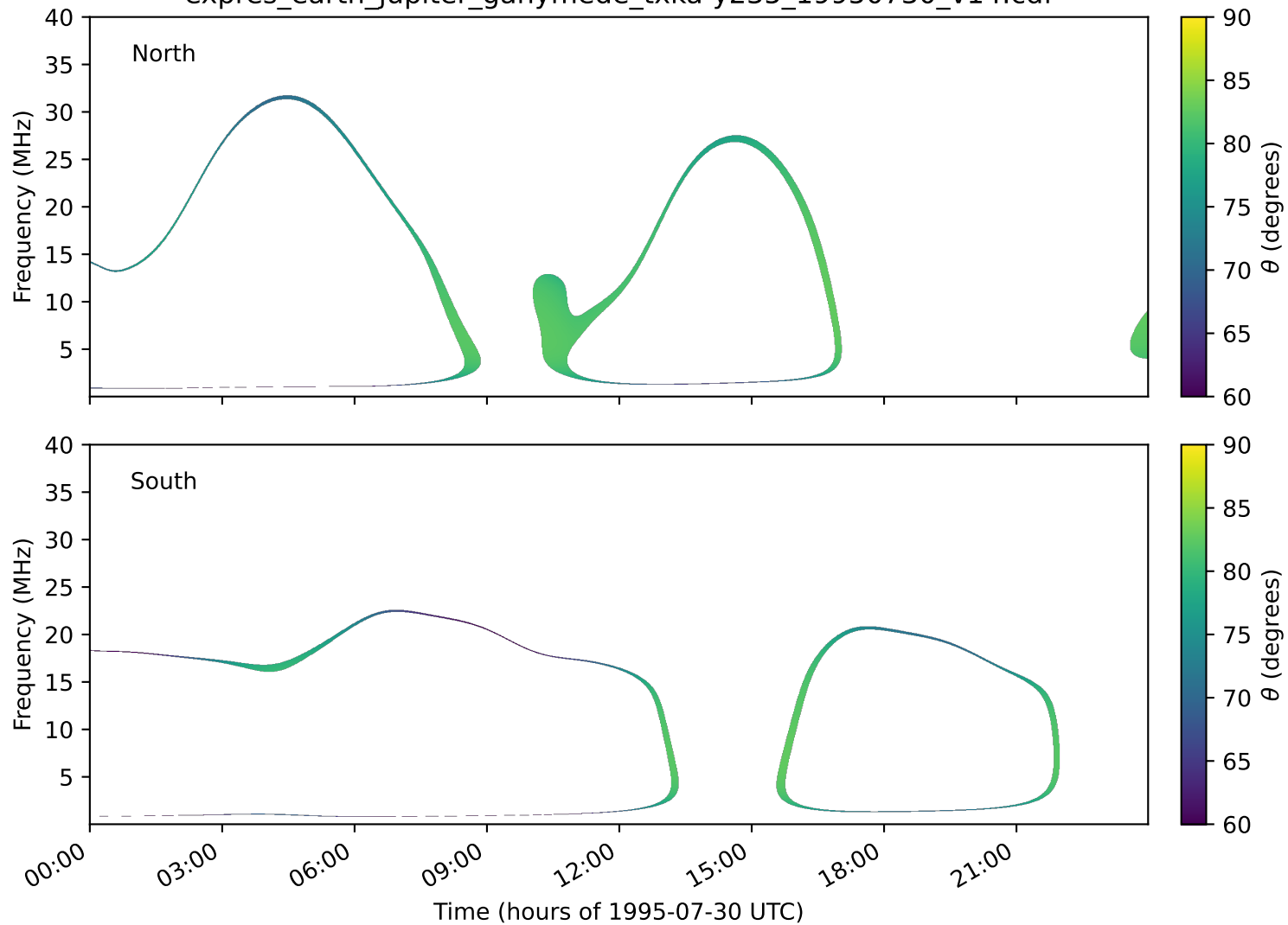
expres_earth_jupiter_ganymede_txka-y235_19950730_v14.cdf
