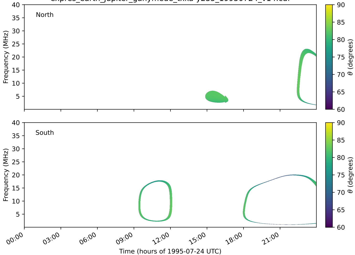
expres_earth_jupiter_ganymede_txka-y235_19950724_v14.cdf
