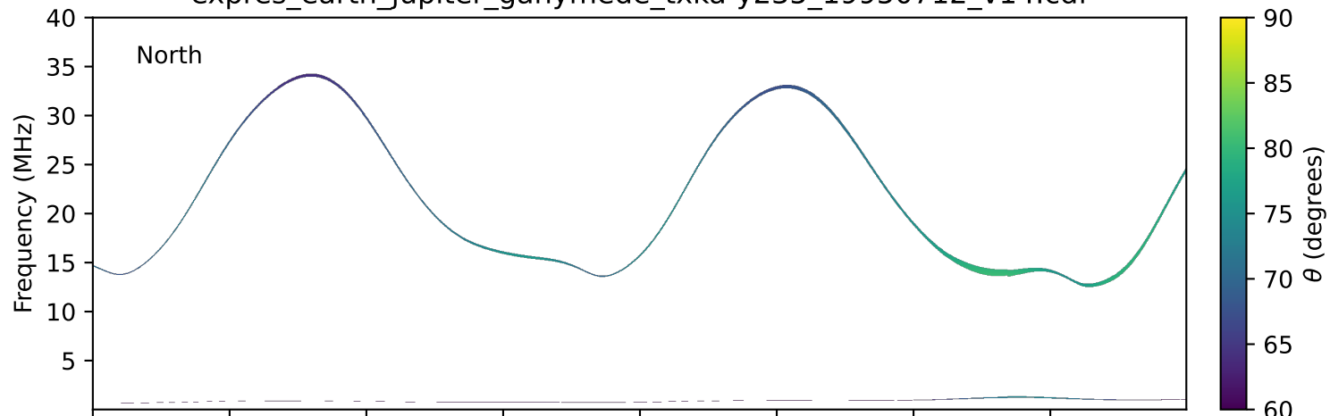
expres_earth_jupiter_ganymede_txka-y235_19950712_v14.cdf
