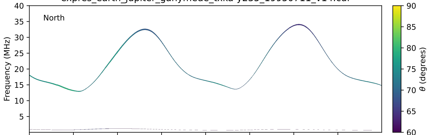
expres_earth_jupiter_ganymede_txka-y235_19950711_v14.cdf
