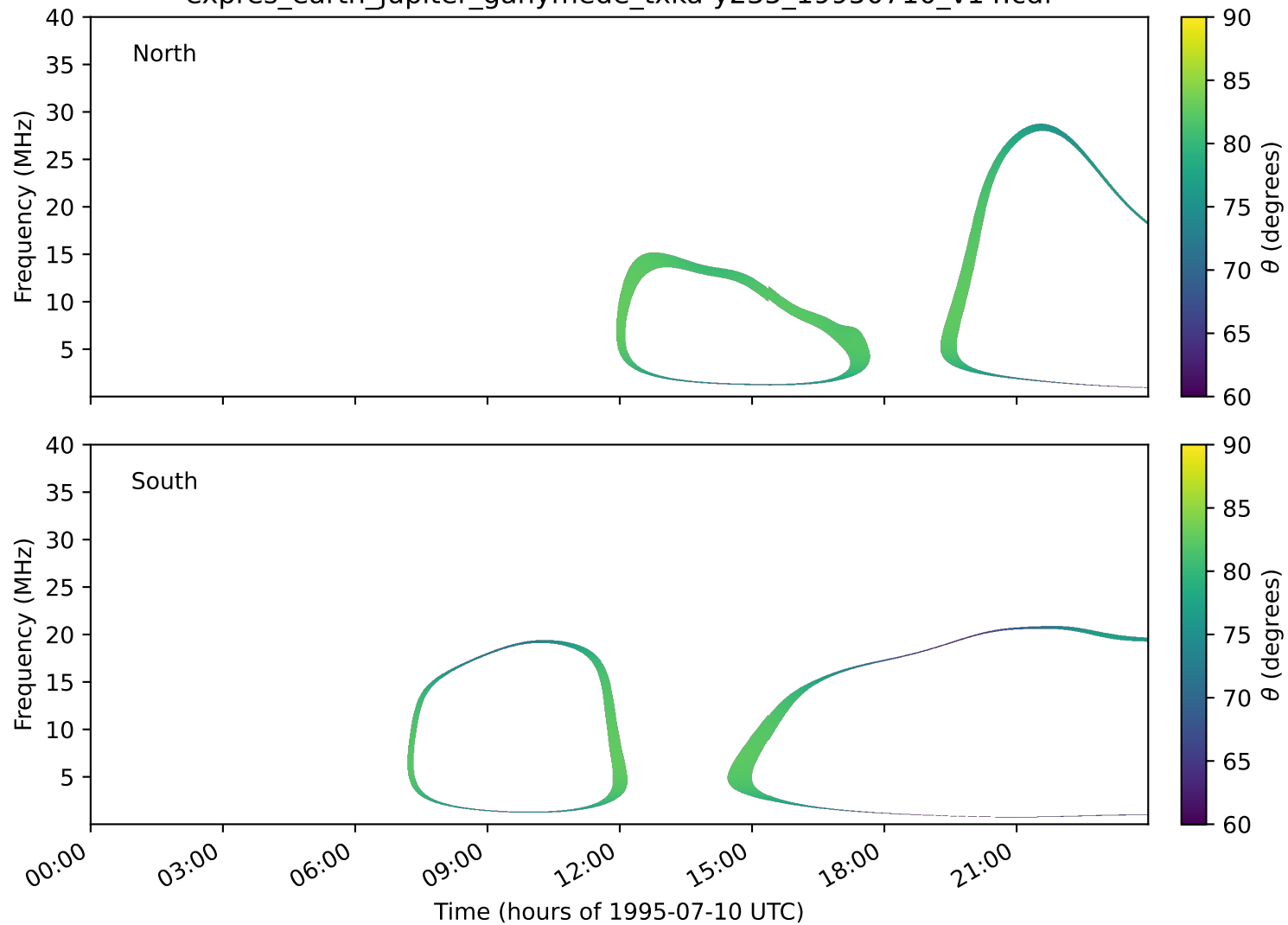
expres_earth_jupiter_ganymede_txka-y235_19950710_v14.cdf
