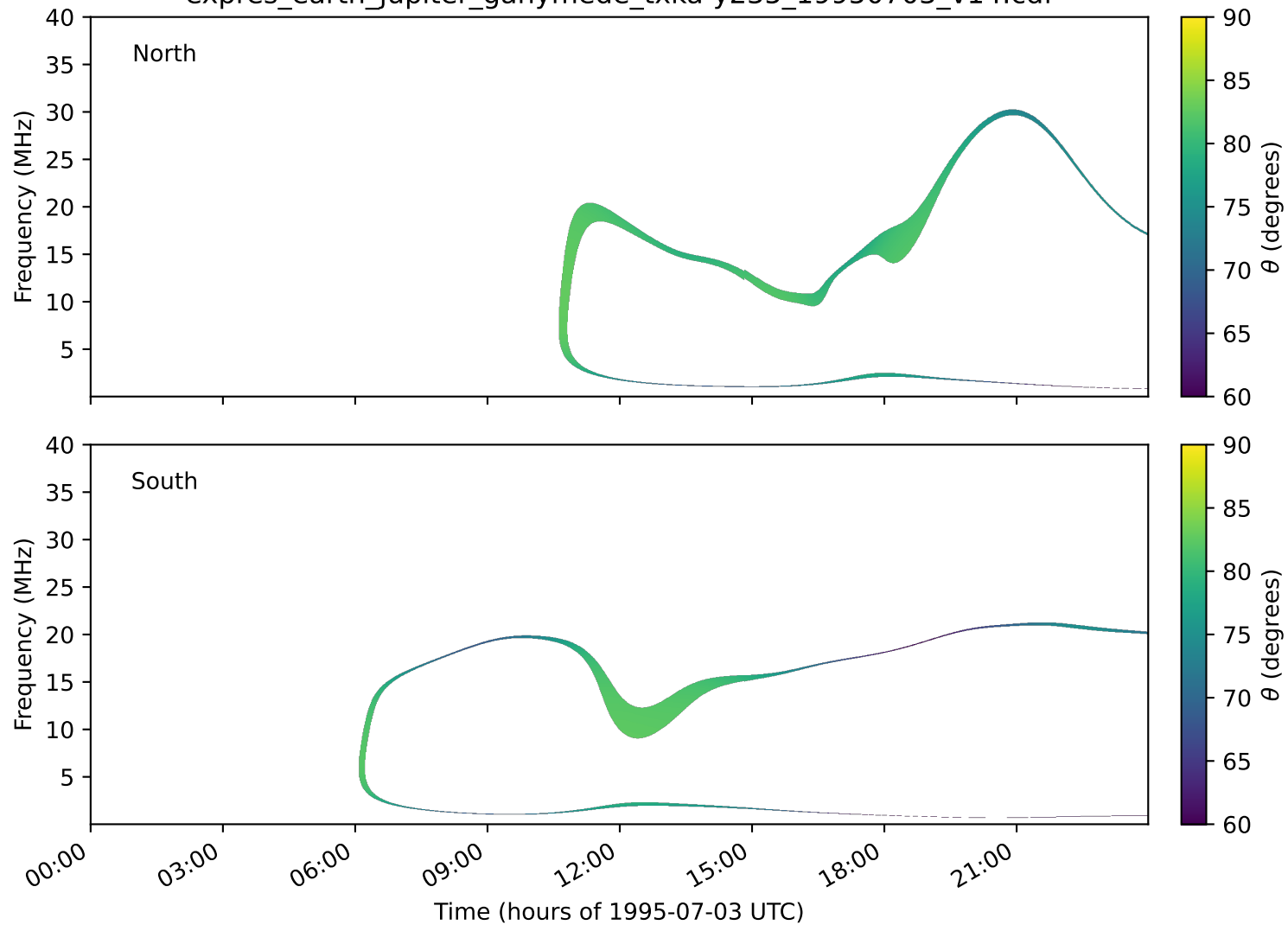
expres_earth_jupiter_ganymede_txka-y235_19950703_v14.cdf
