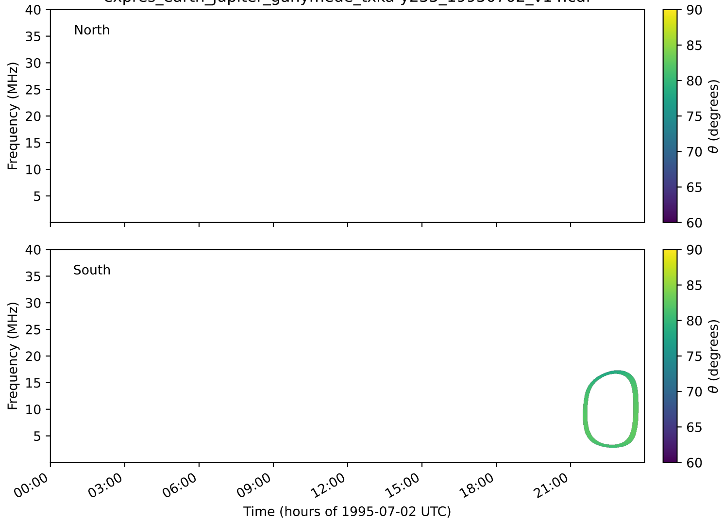
expres_earth_jupiter_ganymede_txka-y235_19950702_v14.cdf
