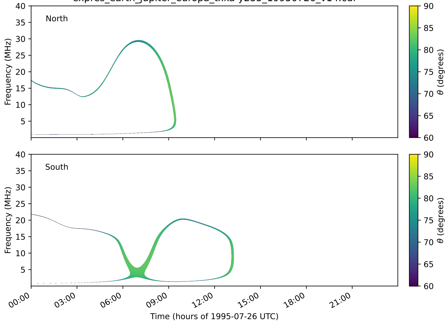
expres_earth_jupiter_europa_txka-y235_19950726_v14.cdf
