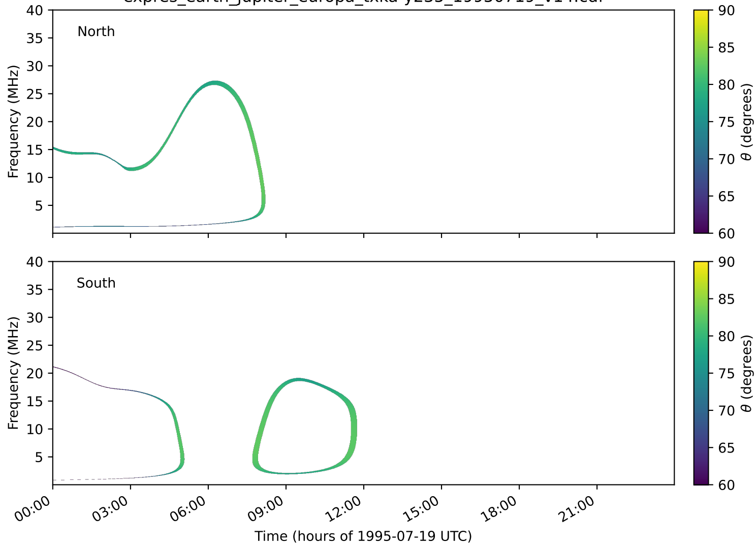
expres_earth_jupiter_europa_txka-y235_19950719_v14.cdf
