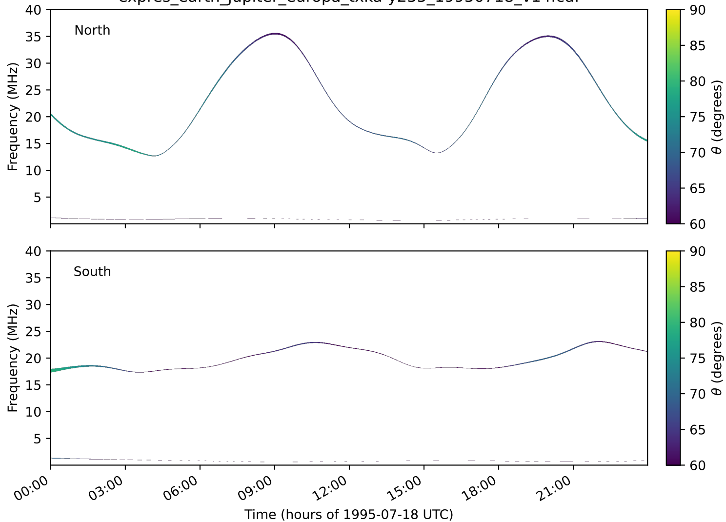
expres_earth_jupiter_europa_txka-y235_19950718_v14.cdf
