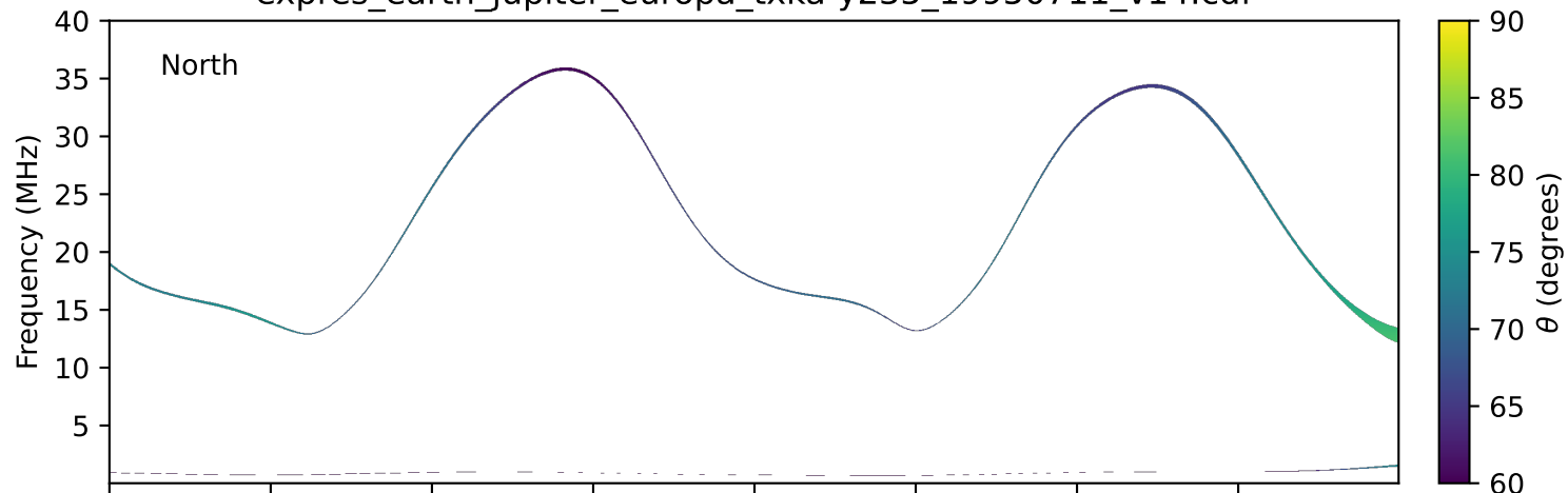
expres_earth_jupiter_europa_txka-y235_19950711_v14.cdf
