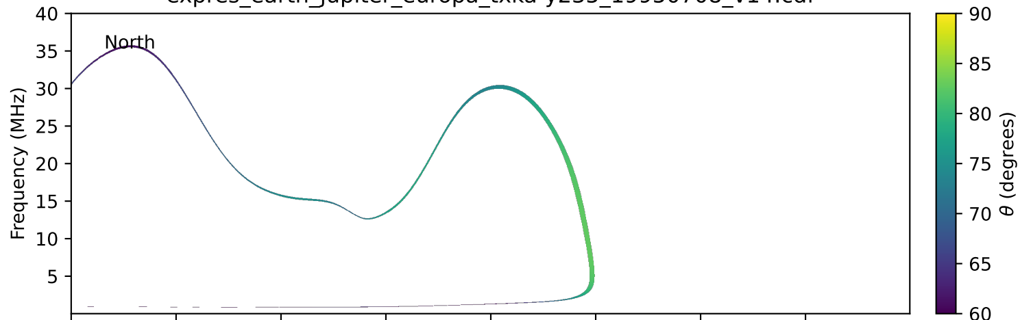
expres_earth_jupiter_europa_txka-y235_19950708_v14.cdf
