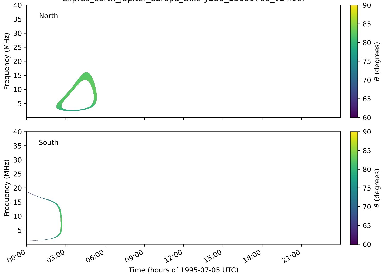
expres_earth_jupiter_europa_txka-y235_19950705_v14.cdf
