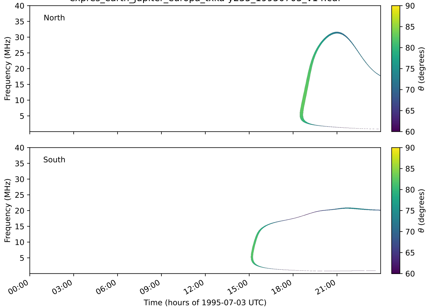
expres_earth_jupiter_europa_txka-y235_19950703_v14.cdf
