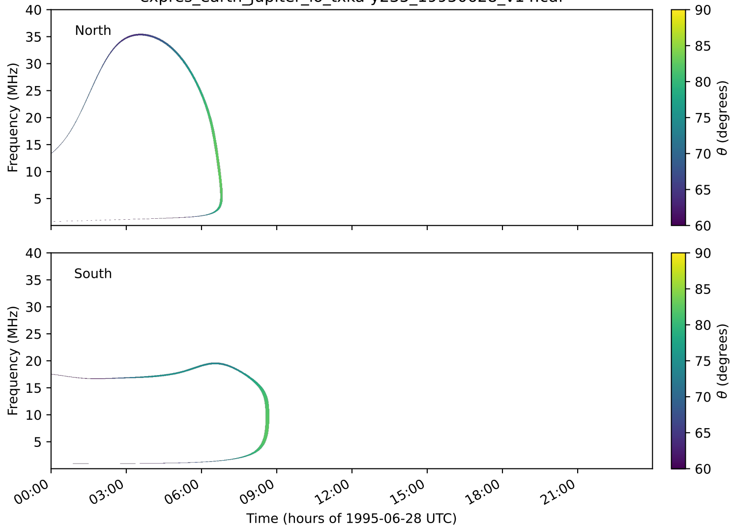
expres_earth_jupiter_io_txka-y235_19950628_v14.cdf
