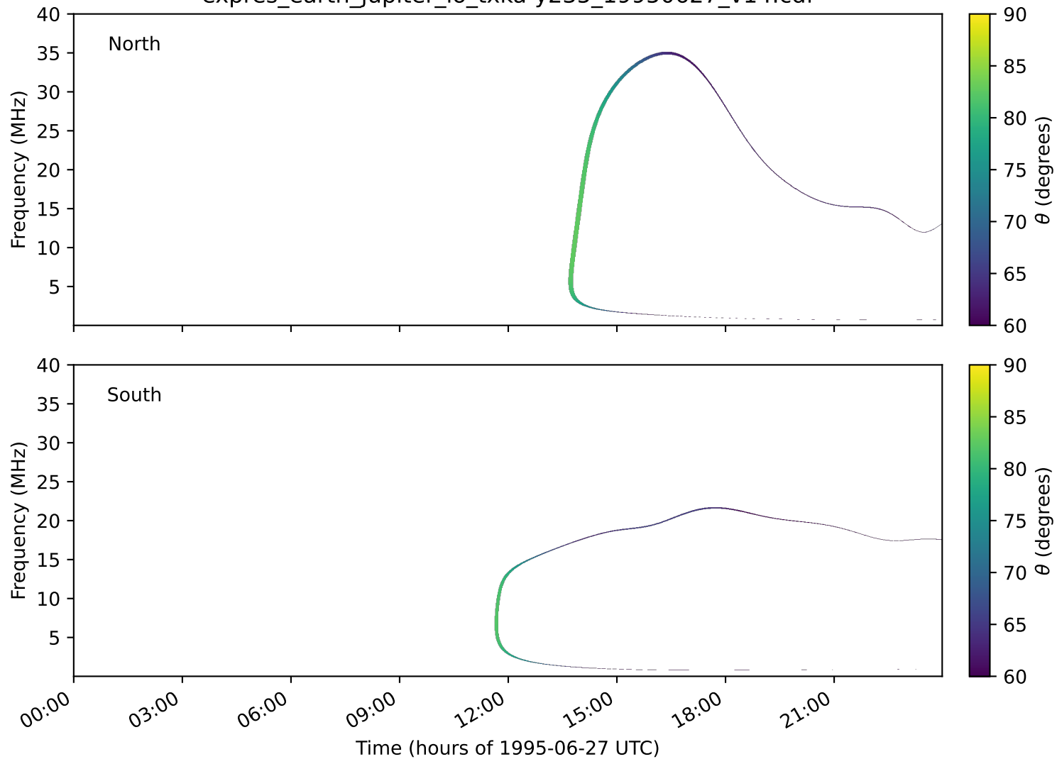
expres_earth_jupiter_io_txka-y235_19950627_v14.cdf
