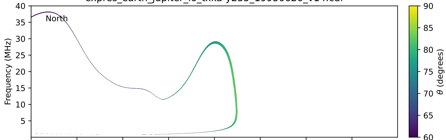
expres_earth_jupiter_io_txka-y235_19950626_v14.cdf
