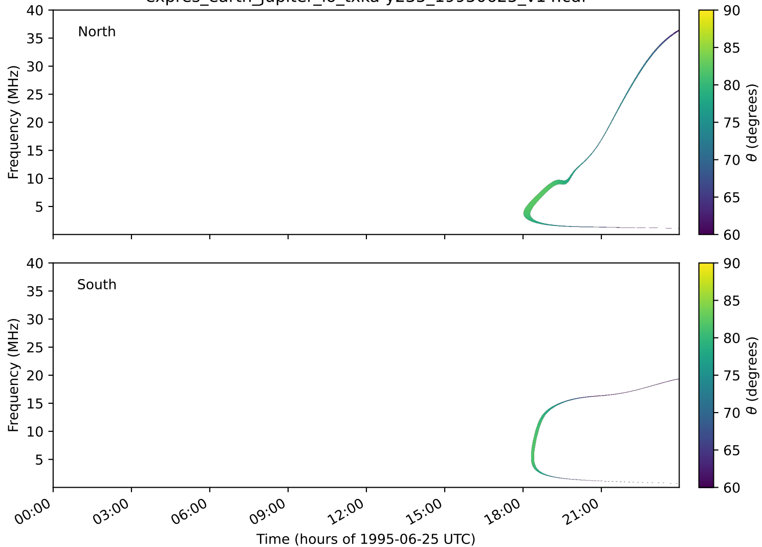
expres_earth_jupiter_io_txka-y235_19950625_v14.cdf
