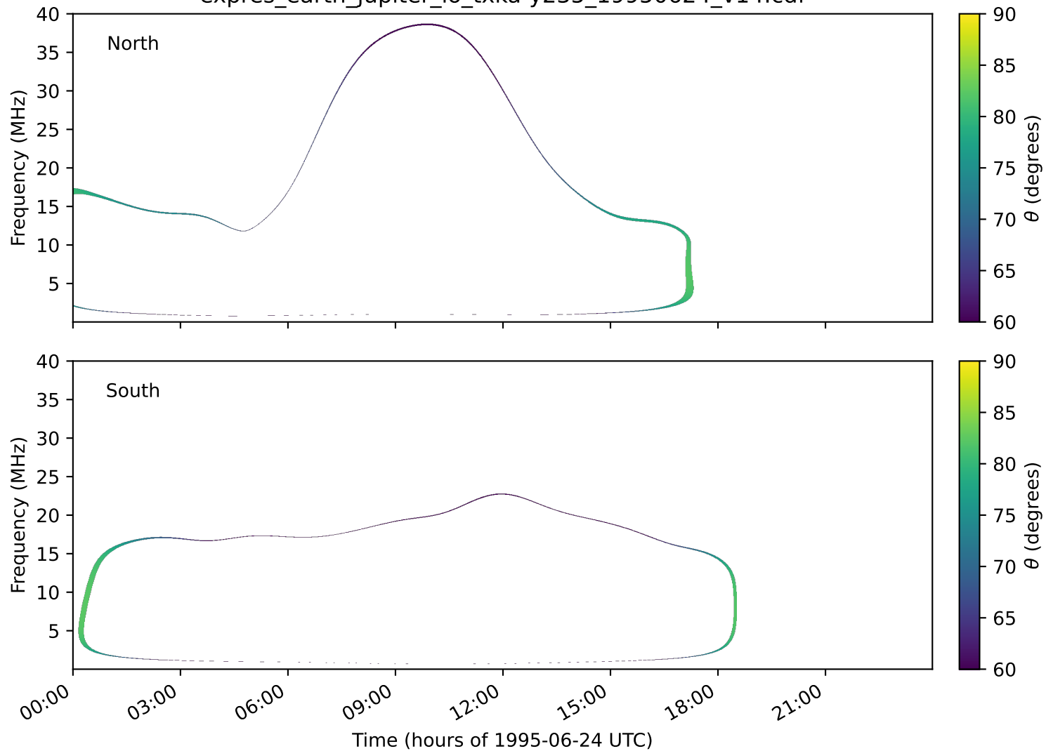
expres_earth_jupiter_io_txka-y235_19950624_v14.cdf
