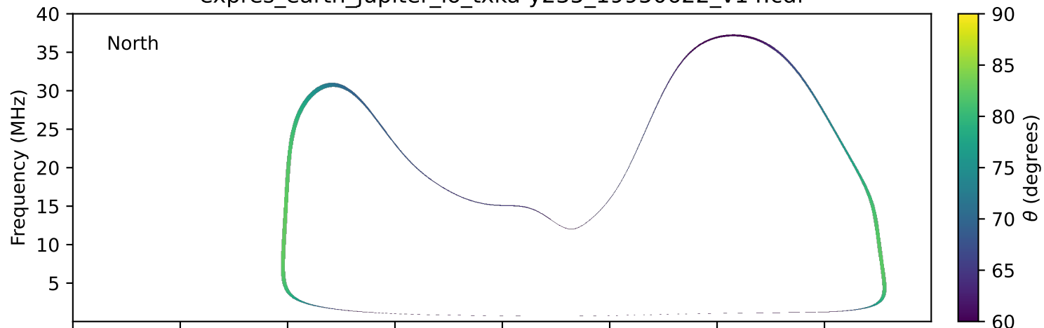
expres_earth_jupiter_io_txka-y235_19950622_v14.cdf
