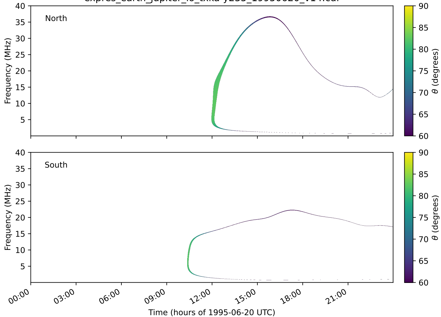
expres_earth_jupiter_io_txka-y235_19950620_v14.cdf
