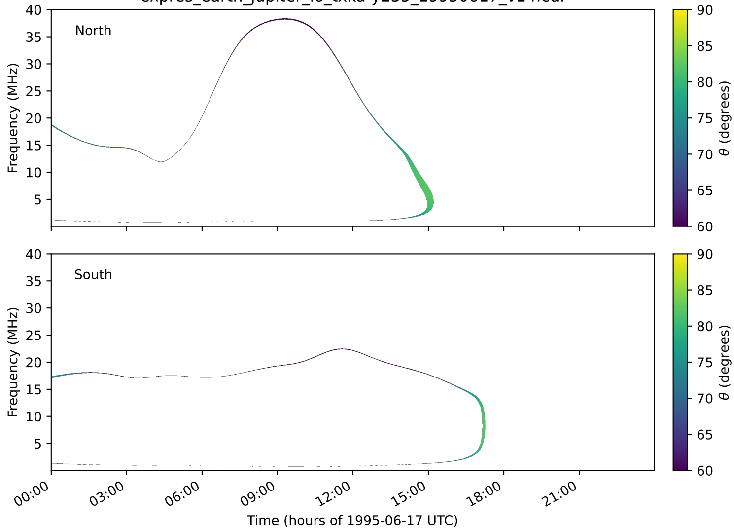
expres_earth_jupiter_io_txka-y235_19950617_v14.cdf
