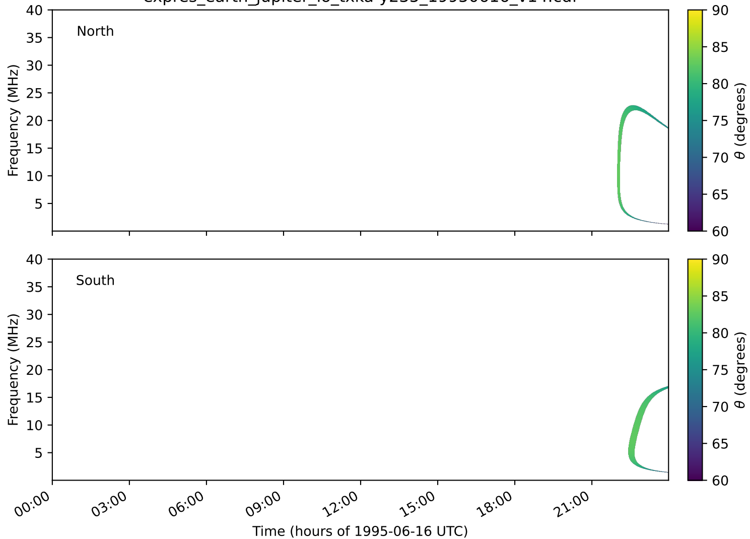
expres_earth_jupiter_io_txka-y235_19950616_v14.cdf
