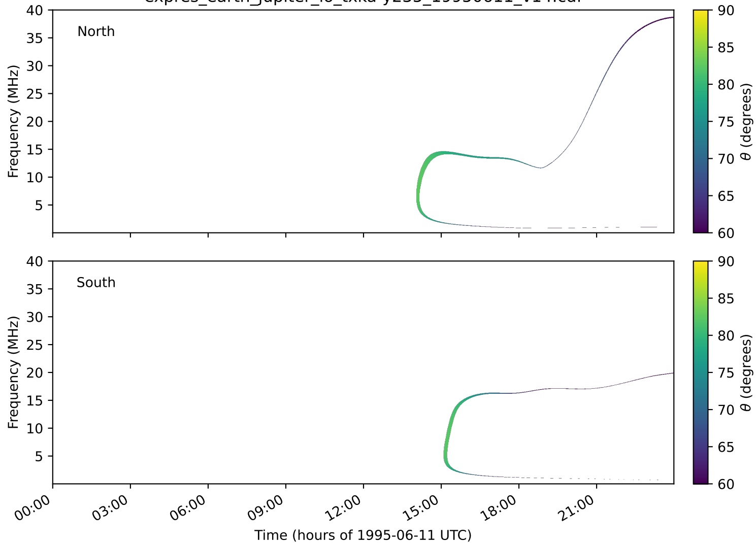
expres_earth_jupiter_io_txka-y235_19950611_v14.cdf
