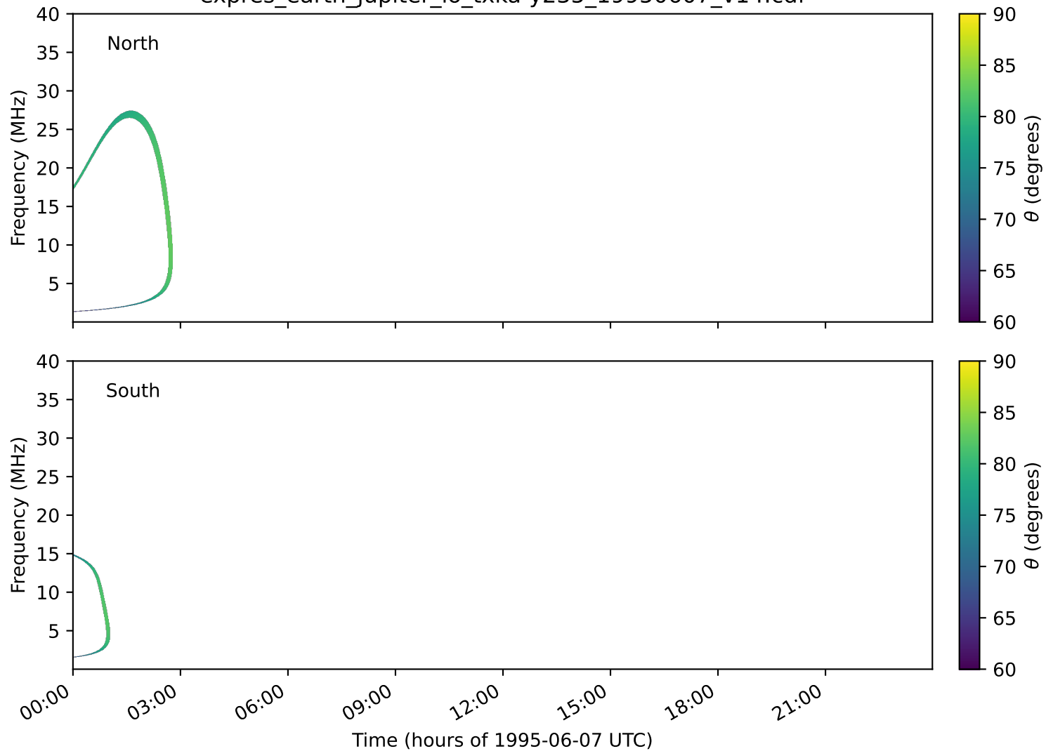
expres_earth_jupiter_io_txka-y235_19950607_v14.cdf
