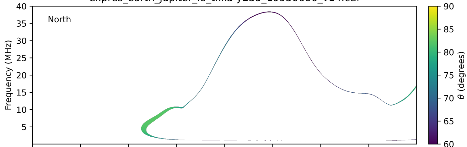
expres_earth_jupiter_io_txka-y235_19950606_v14.cdf
