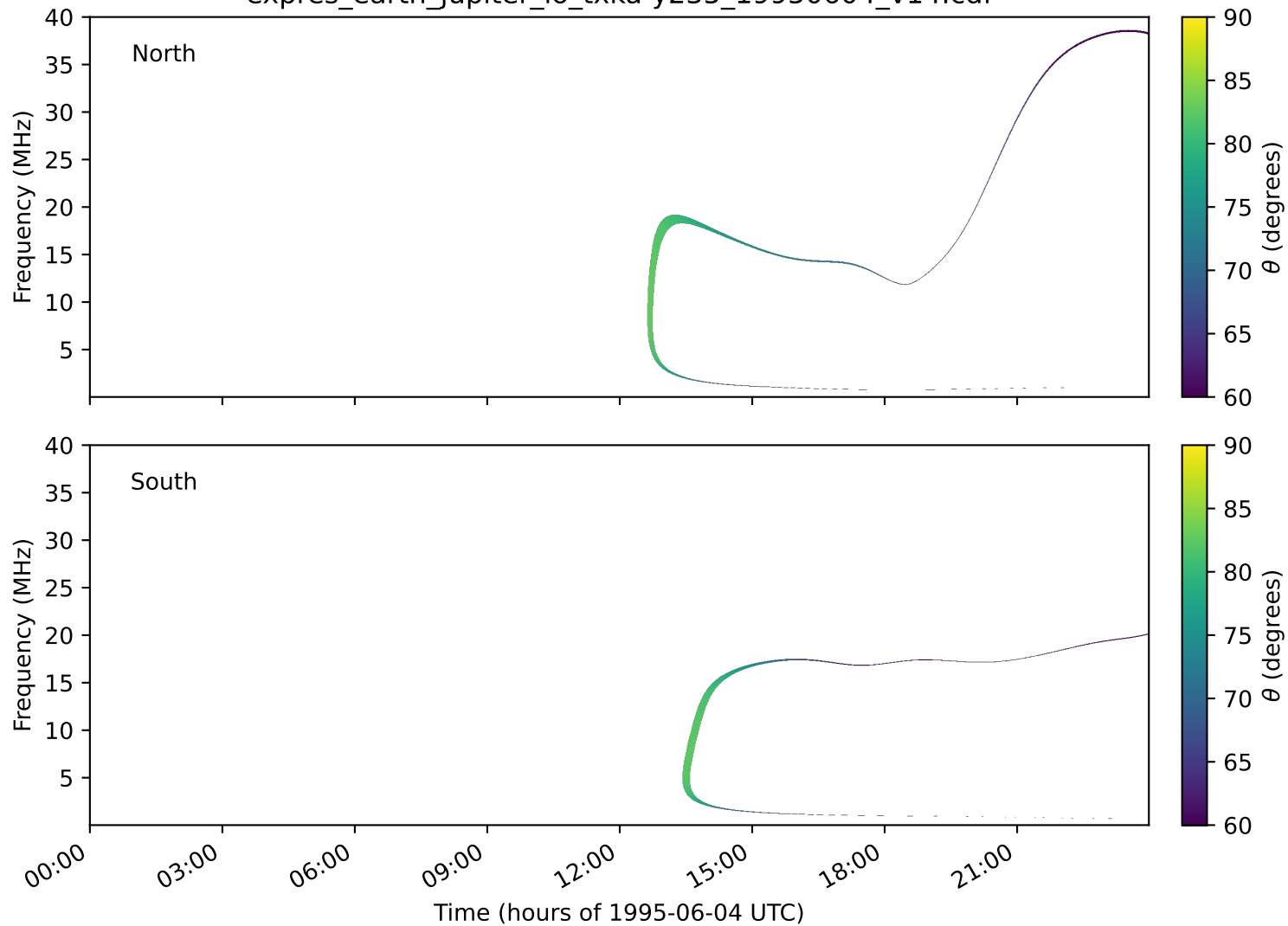
expres_earth_jupiter_io_txka-y235_19950604_v14.cdf
