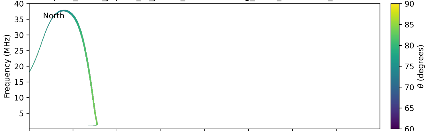
expres_earth_jupiter_io_jrm33_lossc-wid1deg_3kev_19950614_v11.cdf
