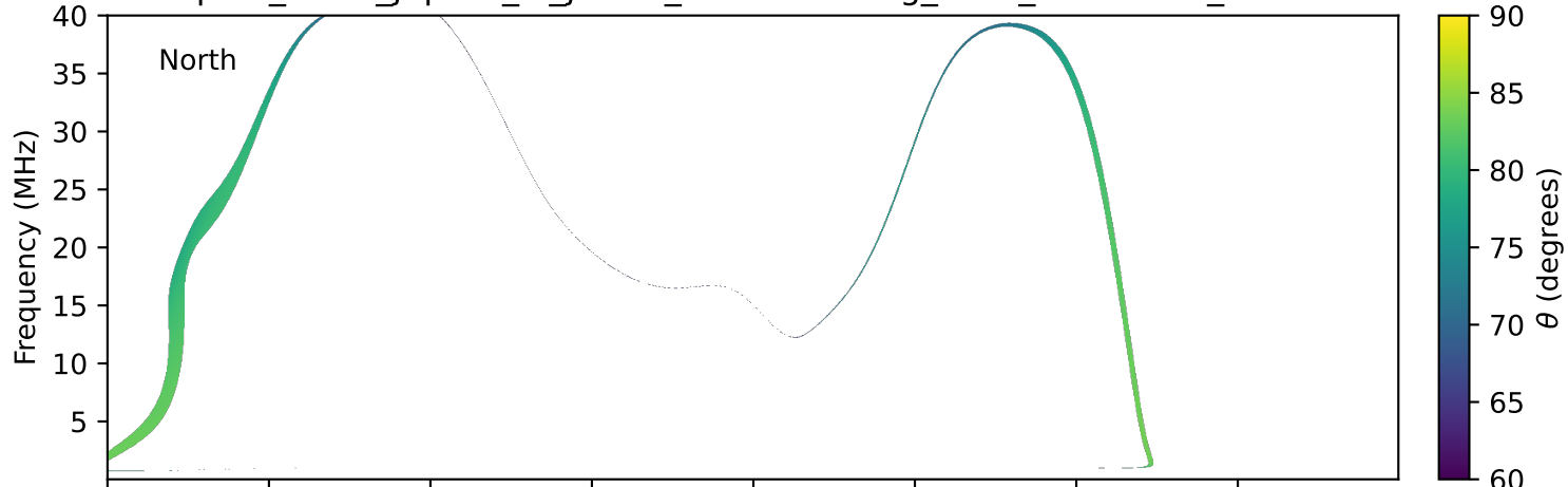
expres_earth_jupiter_io_jrm33_lossc-wid1deg_3kev_19950601_v11.cdf
