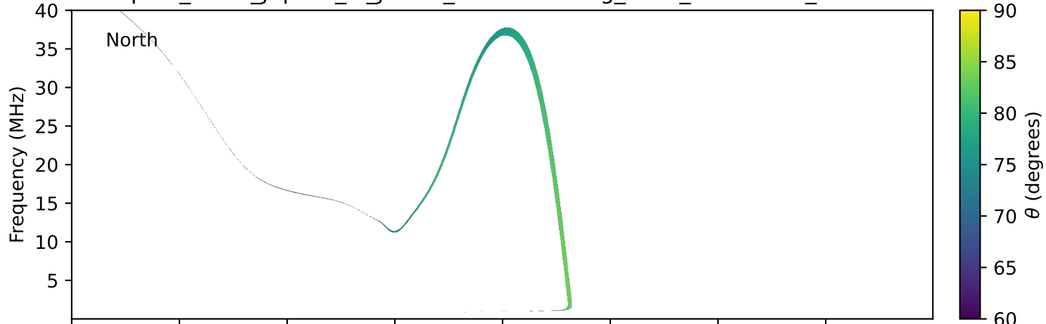
expres_earth_jupiter_io_jrm09_lossc-wid1deg_3kev_19950626_v11.cdf
