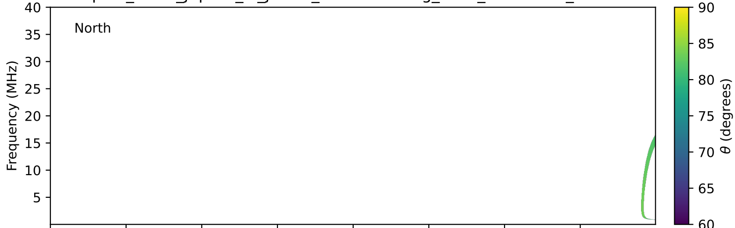
expres_earth_jupiter_io_jrm09_lossc-wid1deg_3kev_19950623_v11.cdf
