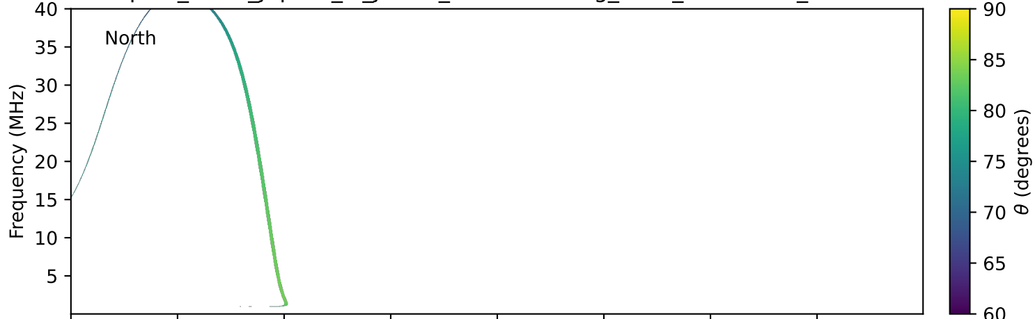
expres_earth_jupiter_io_jrm09_lossc-wid1deg_3kev_19950621_v11.cdf
