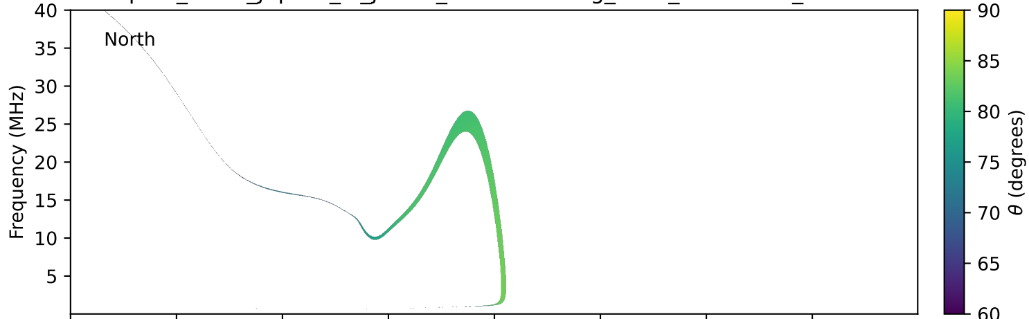
expres_earth_jupiter_io_jrm09_lossc-wid1deg_3kev_19950619_v11.cdf
