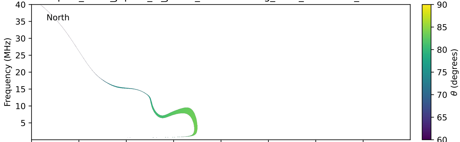
expres_earth_jupiter_io_jrm09_lossc-wid1deg_3kev_19950612_v11.cdf
