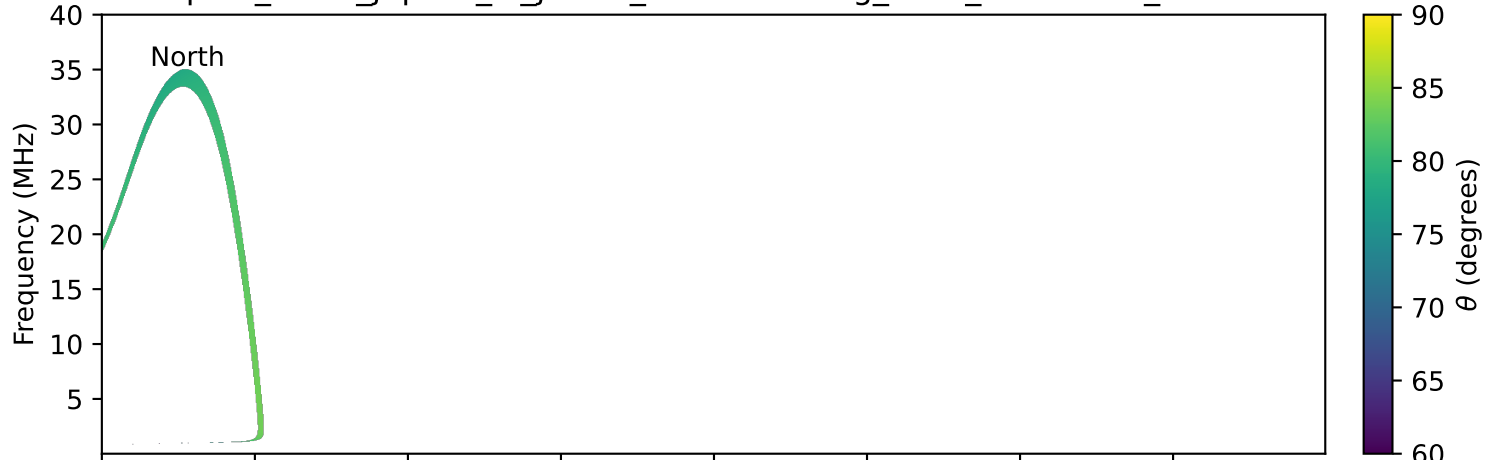
expres_earth_jupiter_io_jrm09_lossc-wid1deg_3kev_19950607_v11.cdf
