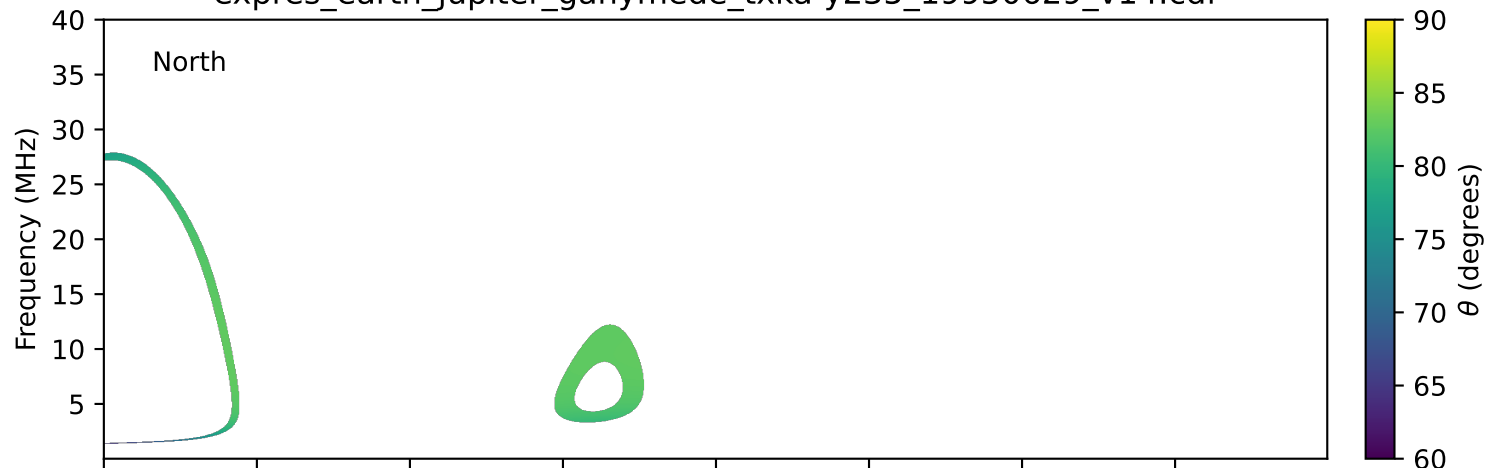
expres_earth_jupiter_ganymede_txka-y235_19950629_v14.cdf
