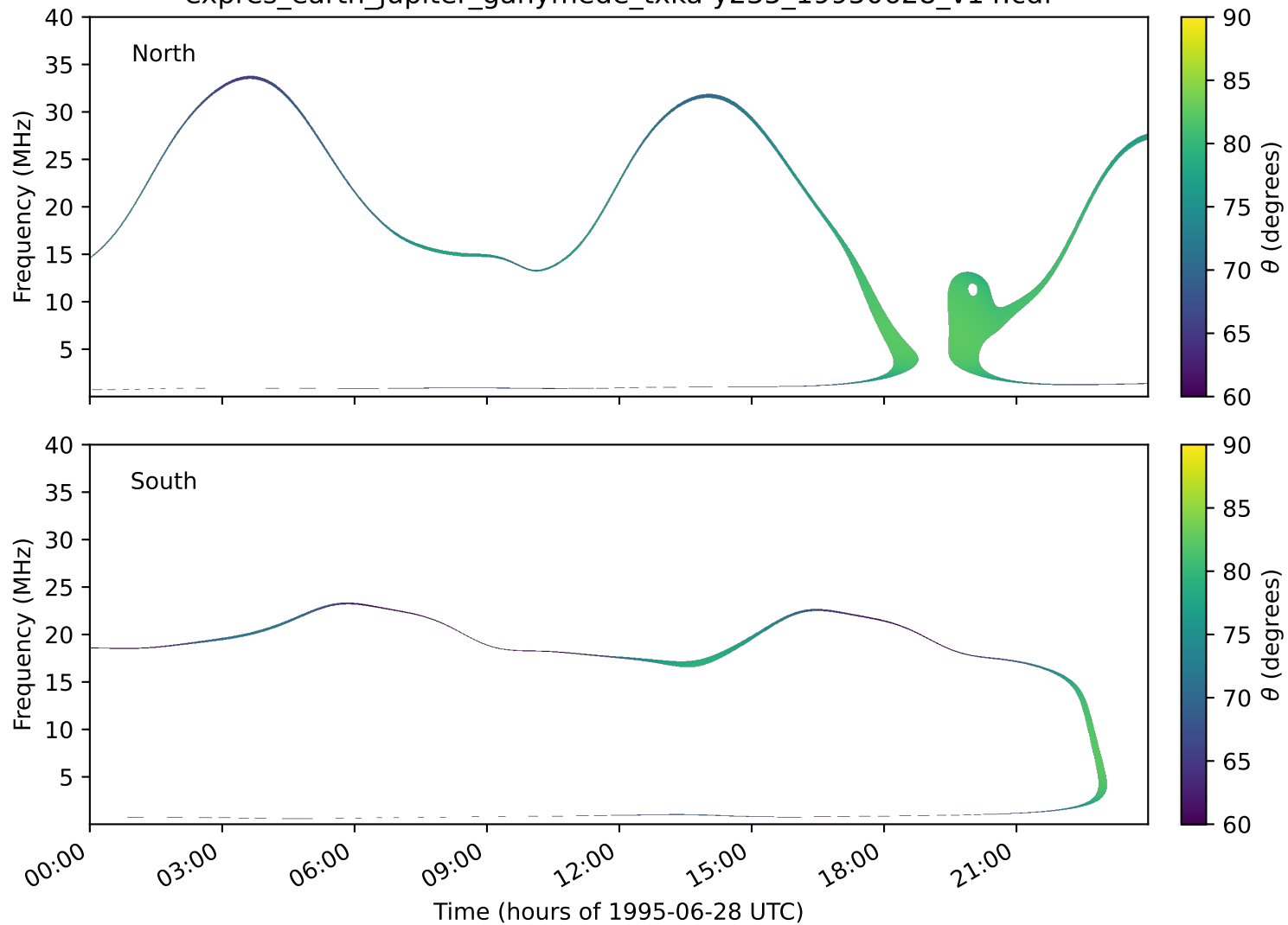
expres_earth_jupiter_ganymede_txka-y235_19950628_v14.cdf
