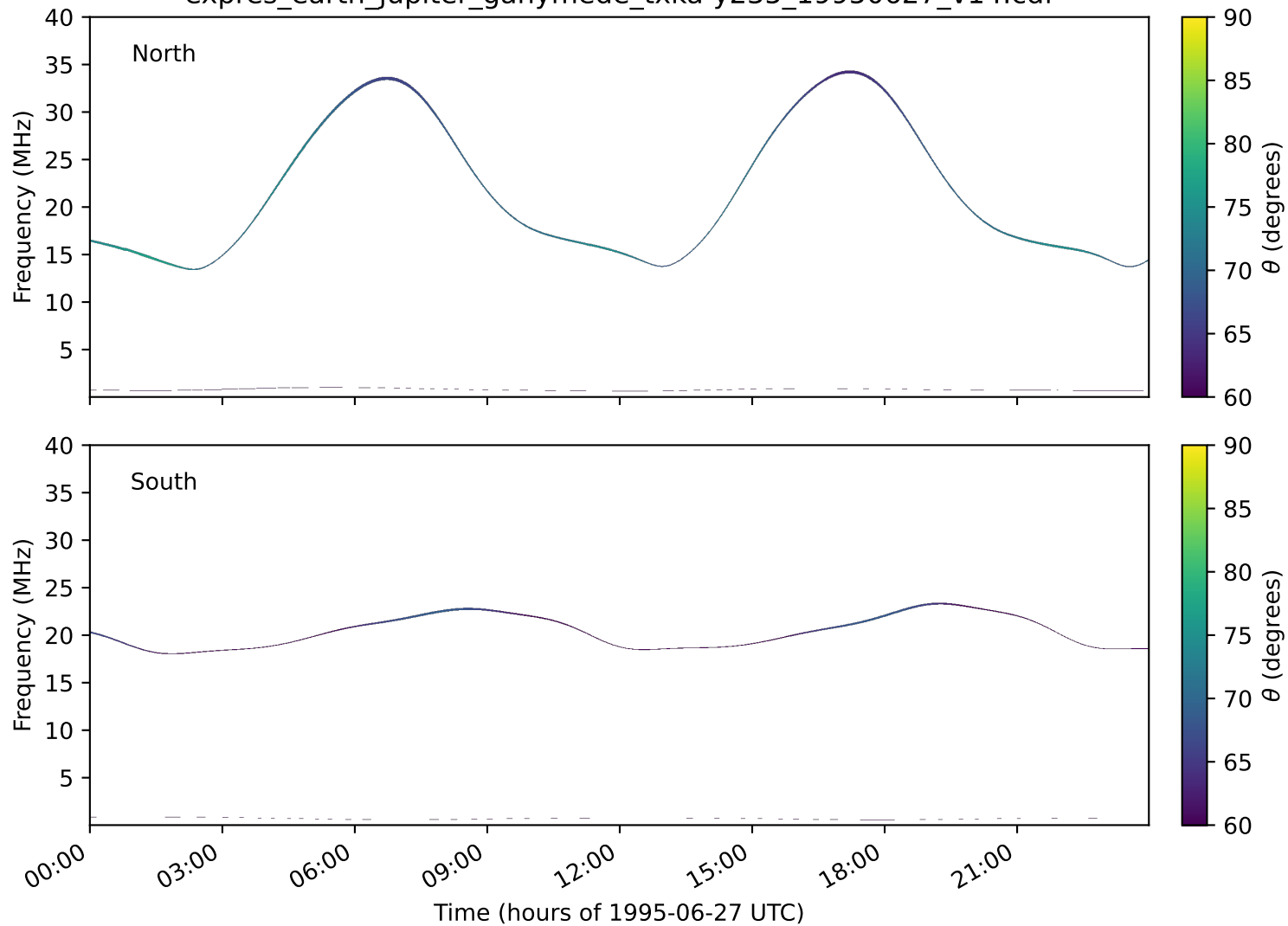
expres_earth_jupiter_ganymede_txka-y235_19950627_v14.cdf
