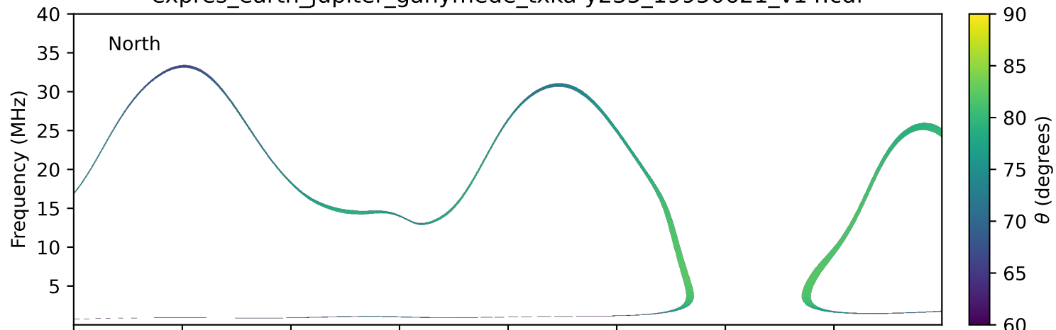
expres_earth_jupiter_ganymede_txka-y235_19950621_v14.cdf
