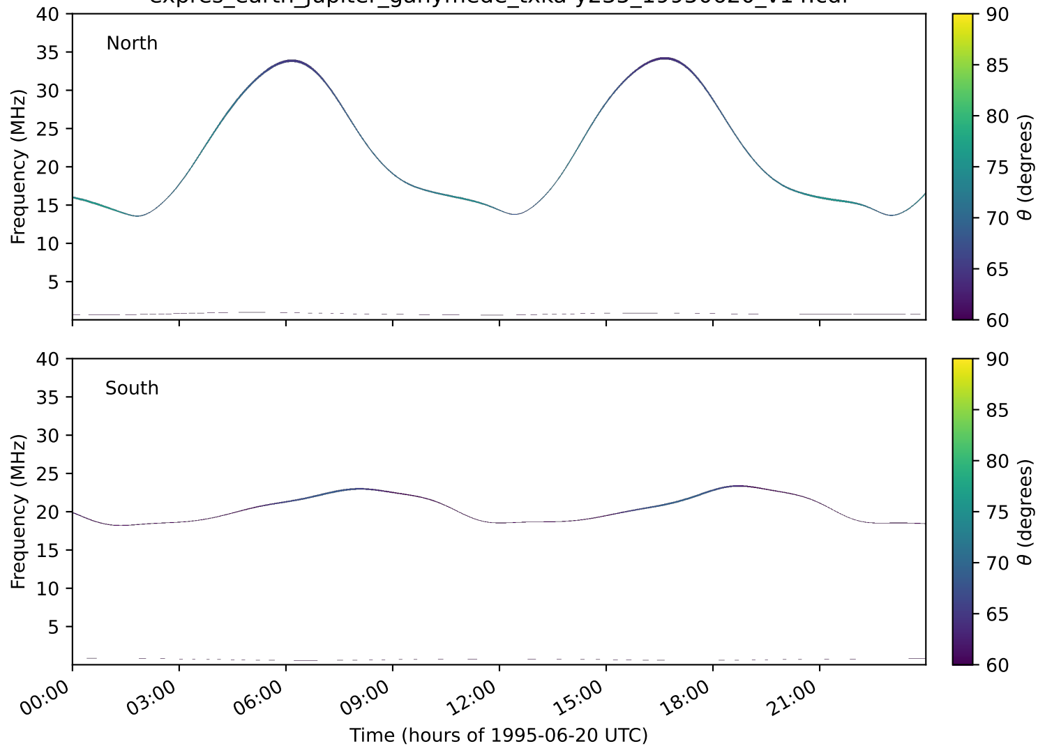
expres_earth_jupiter_ganymede_txka-y235_19950620_v14.cdf
