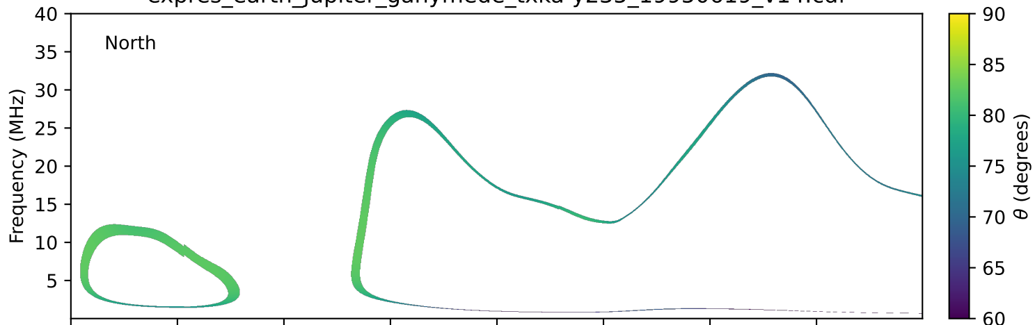
expres_earth_jupiter_ganymede_txka-y235_19950619_v14.cdf
