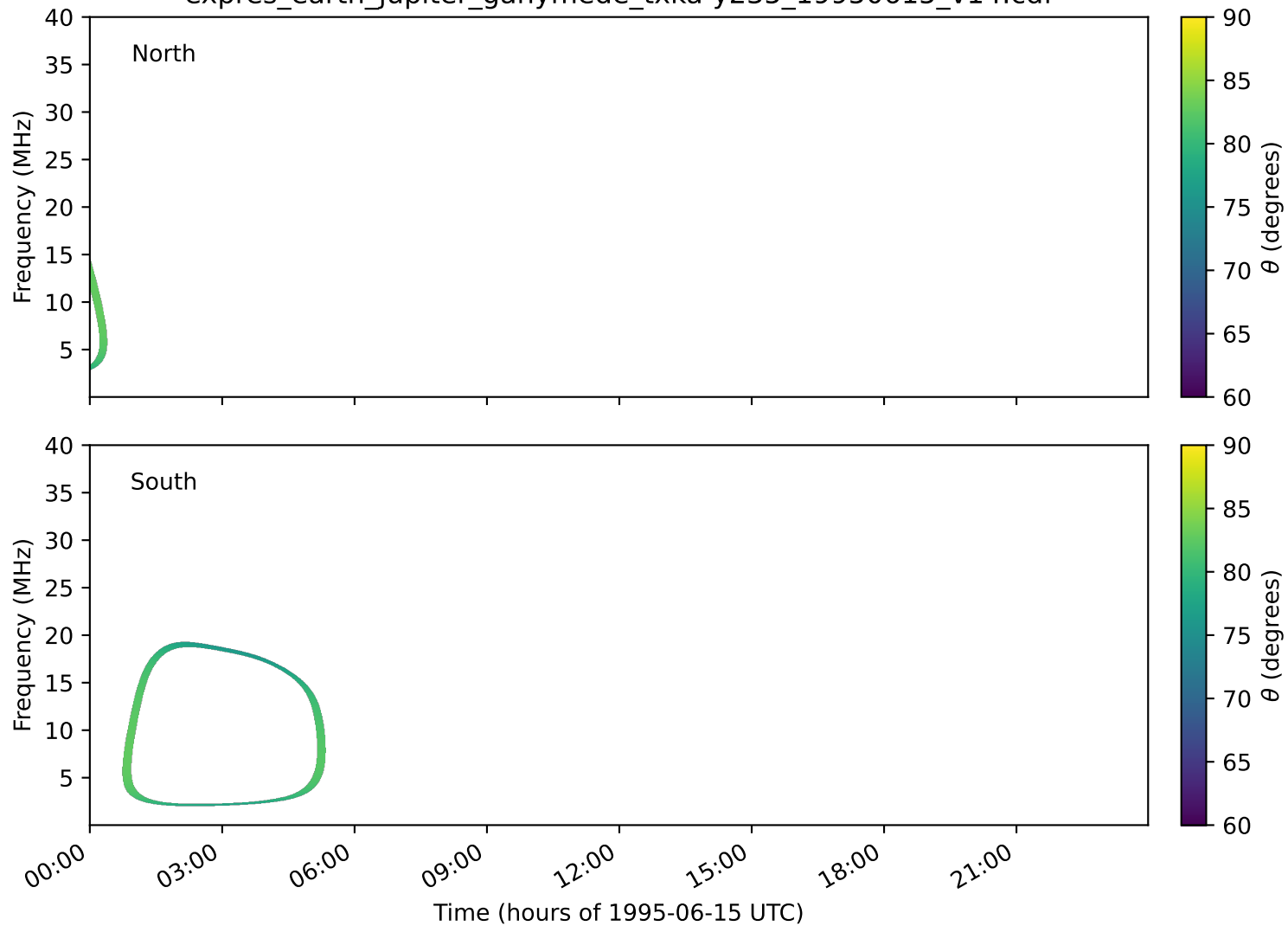
expres_earth_jupiter_ganymede_txka-y235_19950615_v14.cdf
