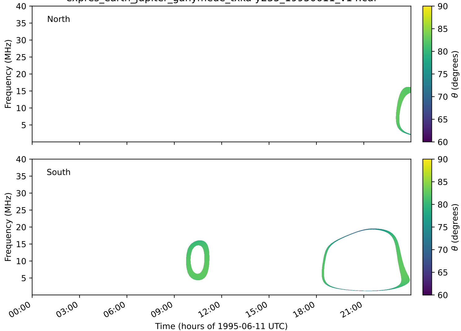
expres_earth_jupiter_ganymede_txka-y235_19950611_v14.cdf
