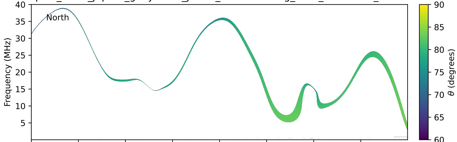
expres_earth_jupiter_ganymede_jrm33_lossc-wid1deg_3kev_19950607_v11.cdf
