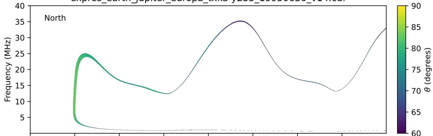
expres_earth_jupiter_europa_txka-y235_19950630_v14.cdf
