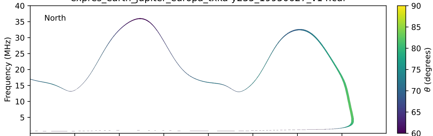
expres_earth_jupiter_europa_txka-y235_19950627_v14.cdf
