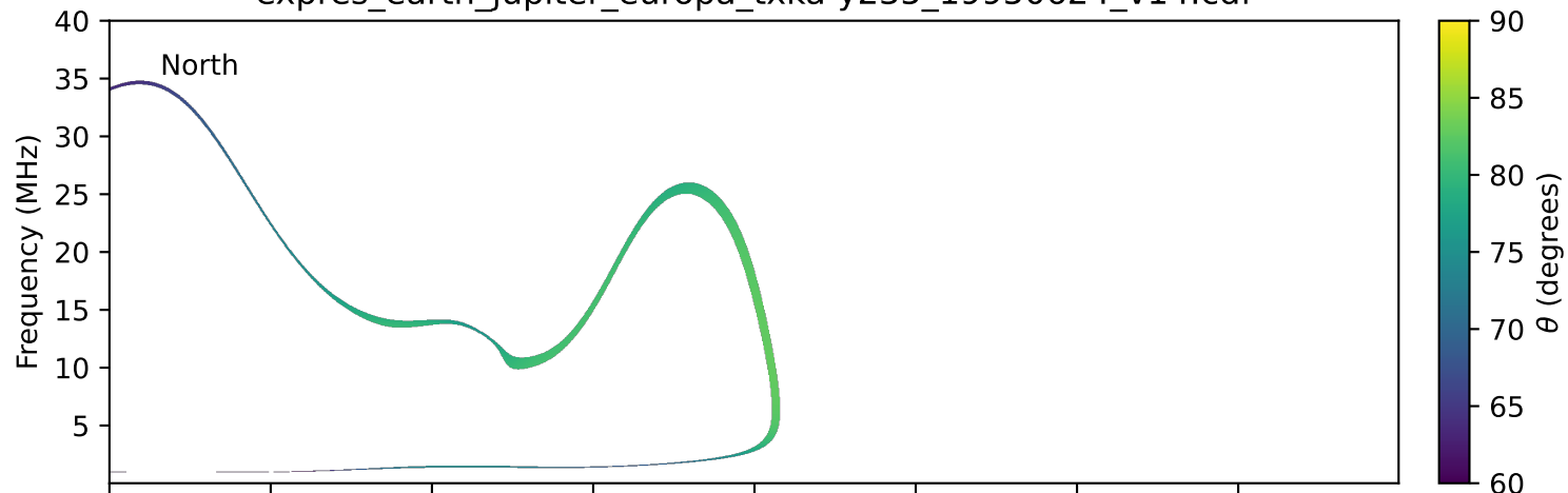
expres_earth_jupiter_europa_txka-y235_19950624_v14.cdf
