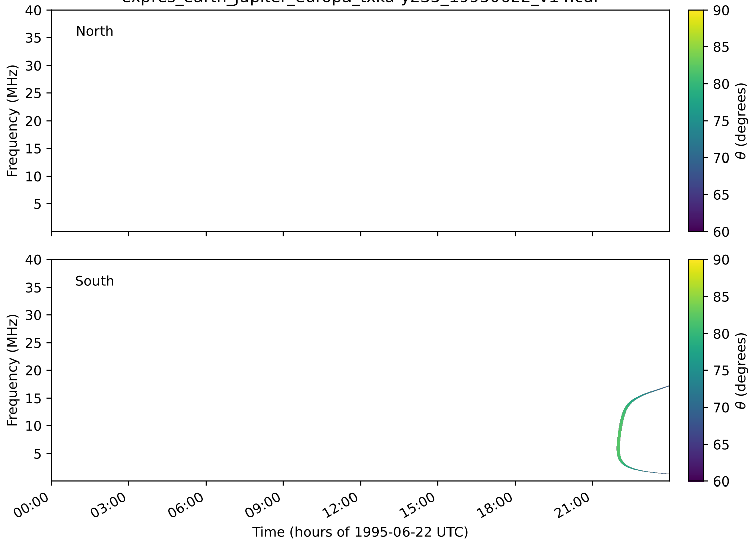
expres_earth_jupiter_europa_txka-y235_19950622_v14.cdf
